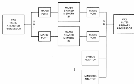
Figure 1-1: A Possible VAX-11/782 System Configuration
